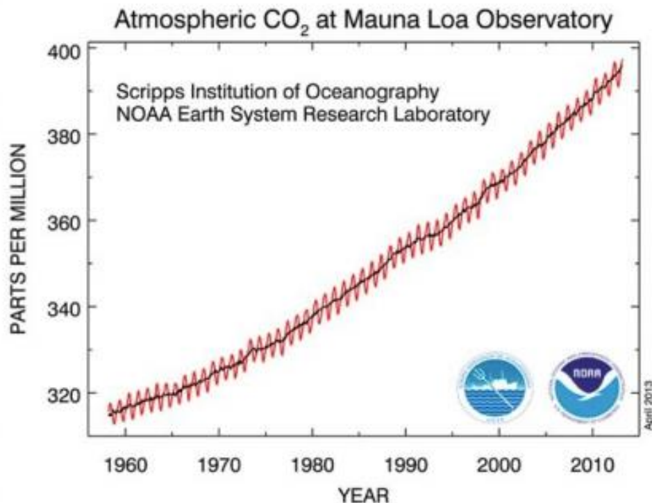
The Keeling Curve, showing CO 2 concentrations increasing to near 400 ppm in 2013. Credit: NOAA.
